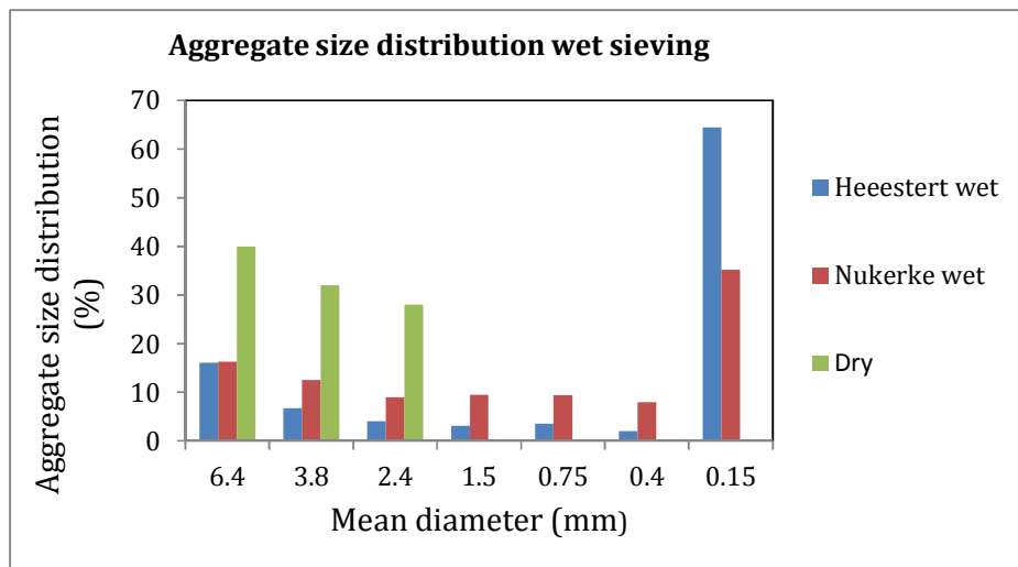
Figure 01: Aggregate distribution (wet sieving) of soil samples.
