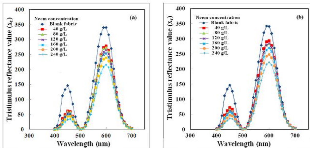
Fig. 12. Variation of the tristimulus reflectance value ( x_r ) with wavelength for neem dyed silk fabrics with different dye bath concentrations before (a) and after (b) exposure to artificial day light for 160 h
