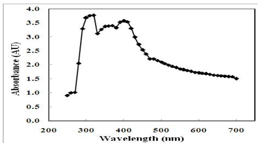
Fig. 2. The absorption spectrum of the aqueous extract of the neem leaves
