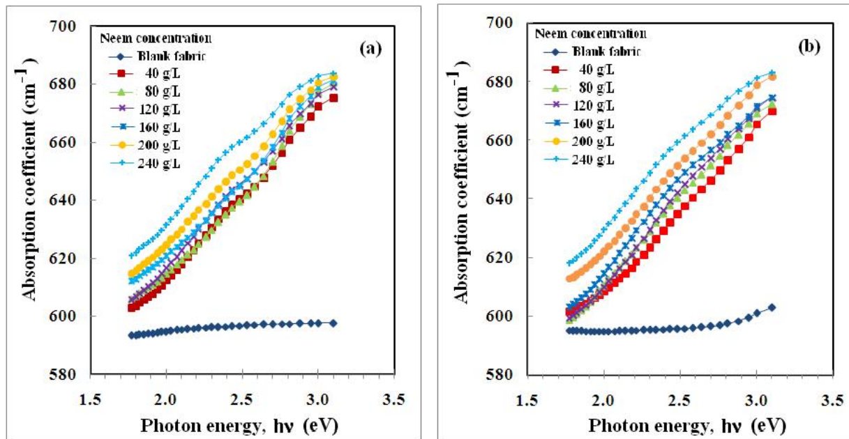
Fig. 5. Plots of the absorption coefficient values of undyed as well as neem silk fabrics with different dye bath concentrations before (a) and after (b) exposure to artificial day light for 160 h against photon energy (hv)
