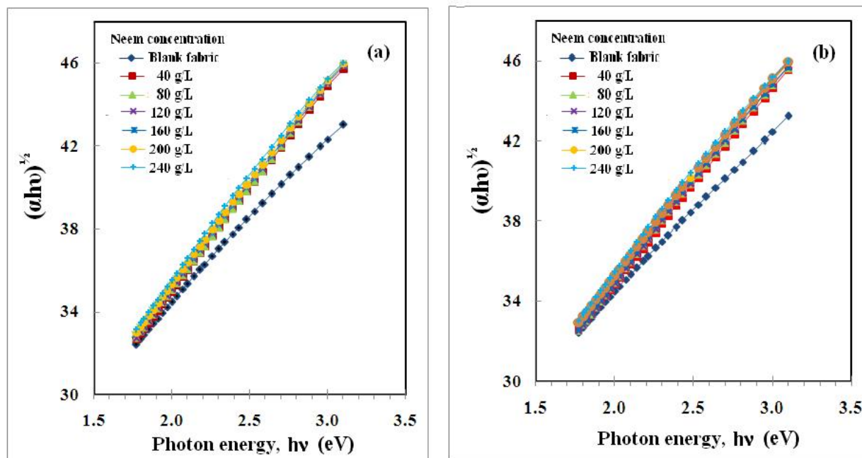
Fig. 8. Variations of (\alpha hv)^{1/2} with photon energy ( hv ) for undyed and neem dyed silk fabrics with different dye bath concentrations before (a) and after (b) exposure to artificial day light for 160 h
