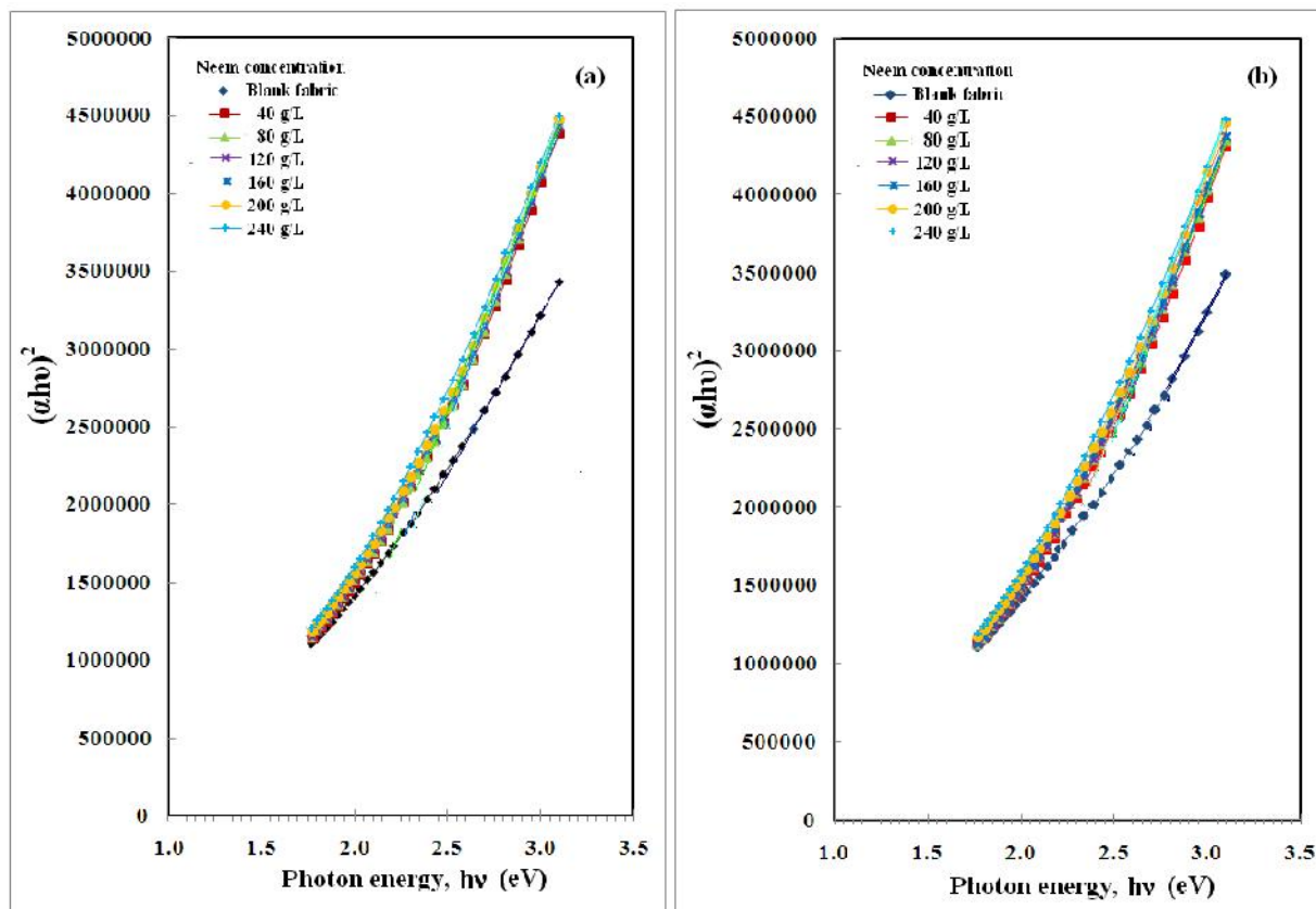
Fig. 7. Variations of (\alpha hv)^2 with photon energy ( h\nu ) for undyed and neem dyed silk fabrics with different dye bath concentrations before (a) and after (b) exposure to artificial day light for 160 h
