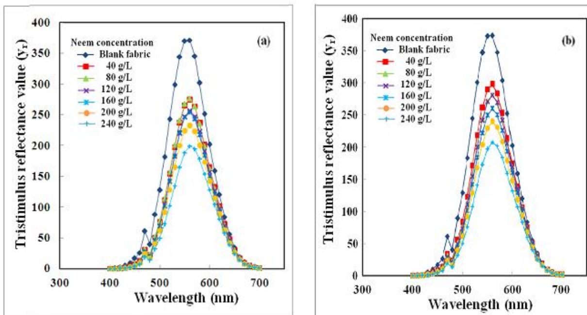
Fig. 13. Variation of the tristimulus reflectance value ( y_T ) with wavelength for neem dyed silk fabrics with different dye bath concentrations before (a) and after (b) exposure to artificial day light for 160 h
