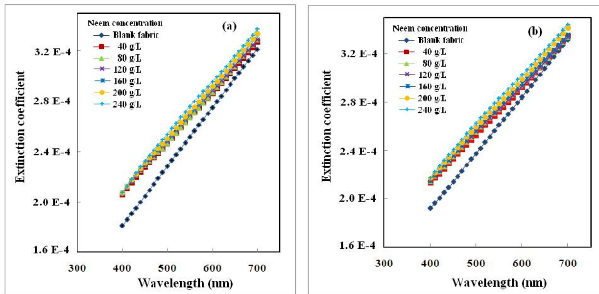
Figure 9: Dependence of the extinction coefficient on wavelength for undyed and neem dyed silk fabrics with different dye bath concentrations before (a) and after (b) exposure to artificial day light for 160 h
