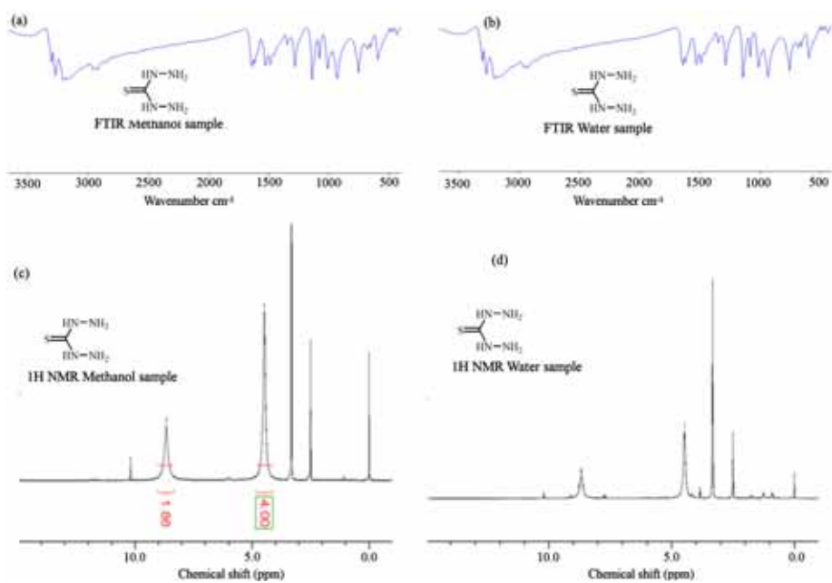
Fig. 1 FTIR and 1 H NMR for thiocarbonylhydrazide prepared through methanol and water synthetic pathways
