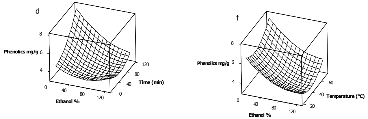
Figure 1: Pair wise response surface plots of the phenolics (mg GAE/g DW) extraction from Passiflora edulis leaves as a function of ethanol %, extraction temperature and time: ethanol % was kept constant at 30% (a) and 100% (b); temperature of extraction was kept constant at 30 °C (c) and 60 °C (d); the time of extraction was kept constant at 30 min (e) and 90 min (f).
