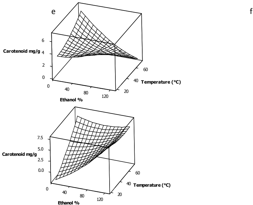
Figure 2: Pair wise response surface plots of the carotenoids (mg/g DW) extraction from Passiflora edulis leaves as a function of ethanol %, extraction temperature, and time: ethanol % was kept constant at 30% (a) and 100% (b); temperature of extraction was kept constant at 30 °C (c) and 60 °C (d); the time of extraction was kept constant at 30 min (e) and 90 min (f).
